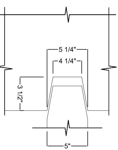
SECTION B
